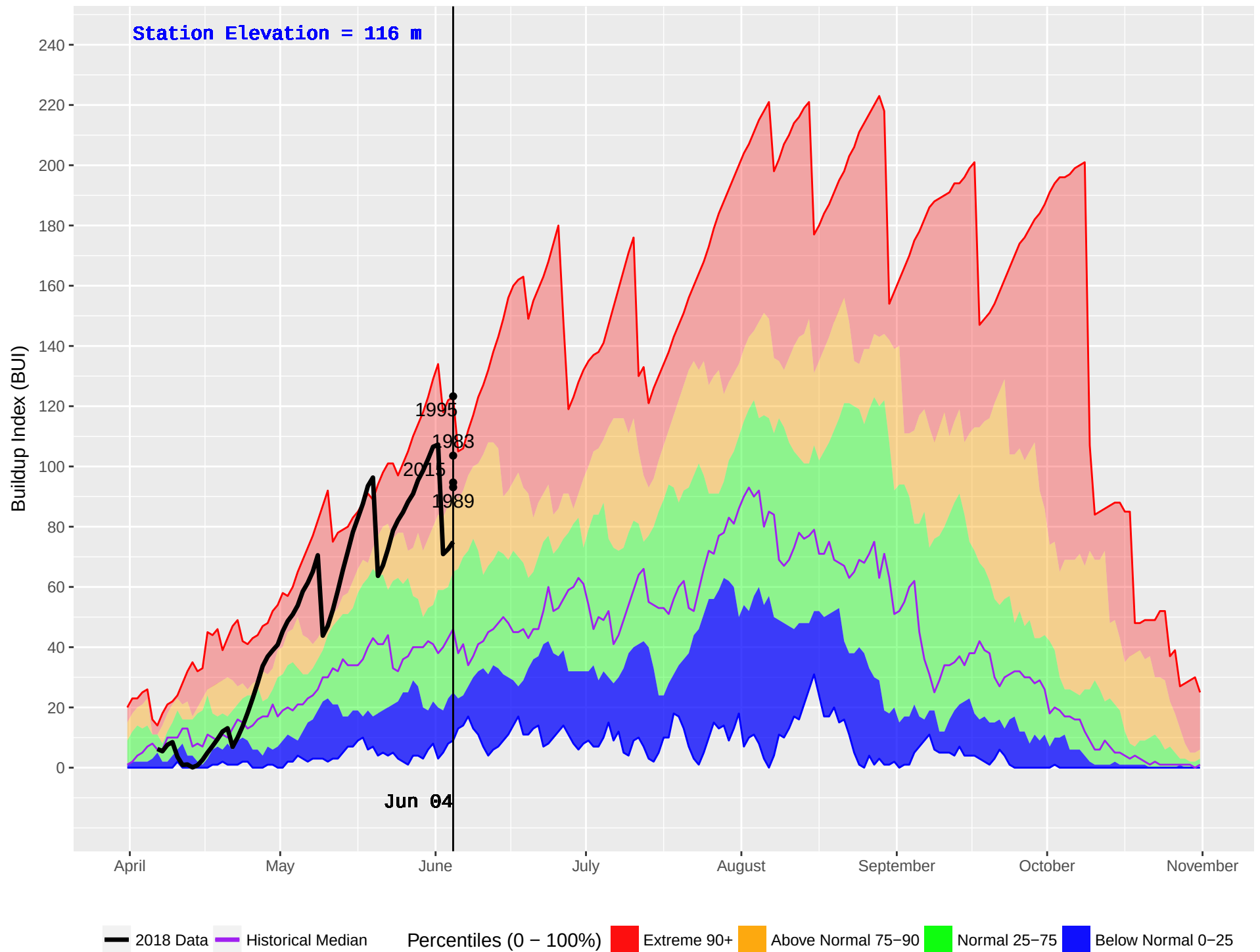
SCAR CREEK (82) : Historical (1982–2016) and Current (2018) Noon Buildup Index (BUI)
