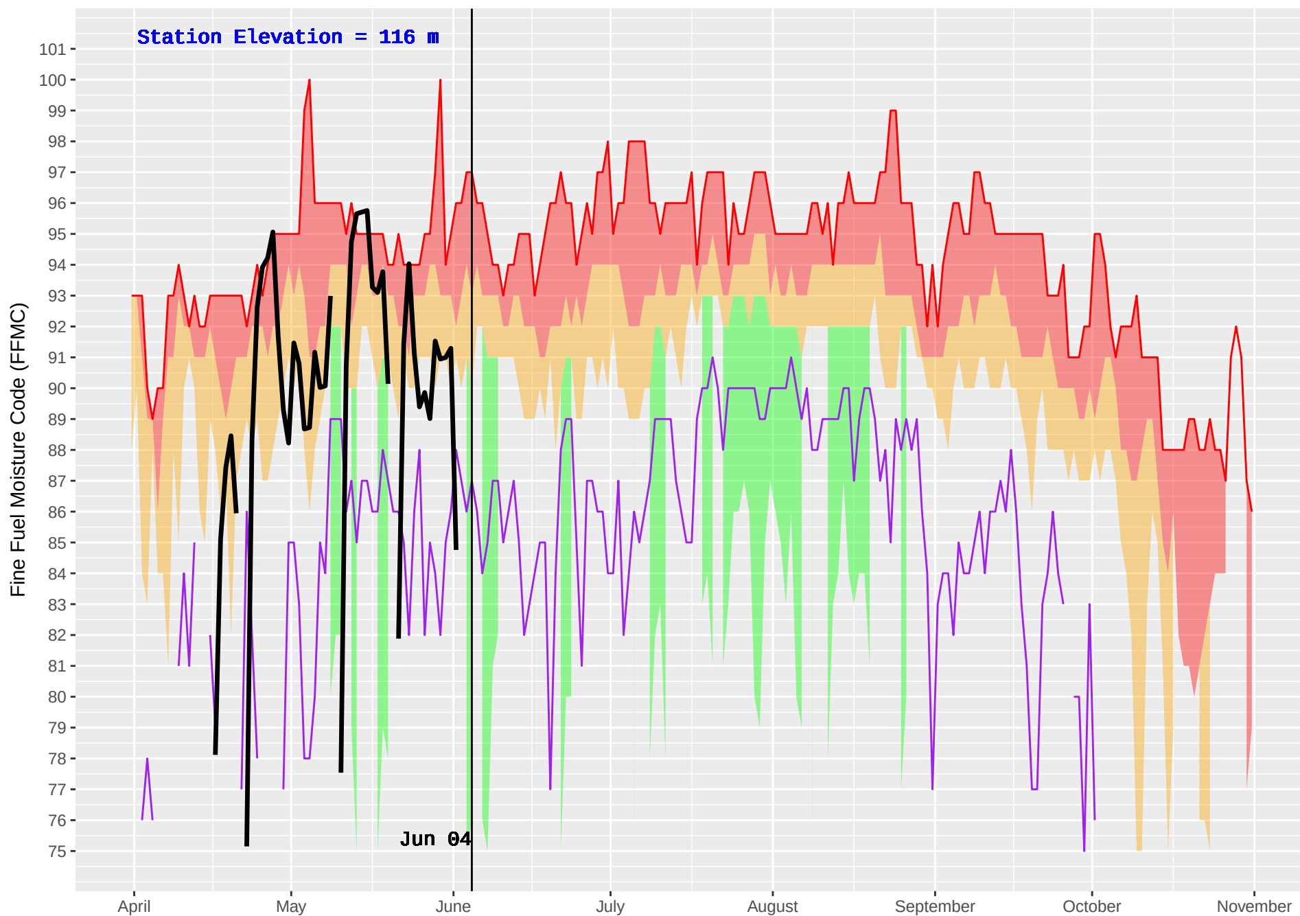
SCAR CREEK (82) : Historical (1982–2016) and Current (2018) Noon Fine Fuel Moisture Code (FFMC)
