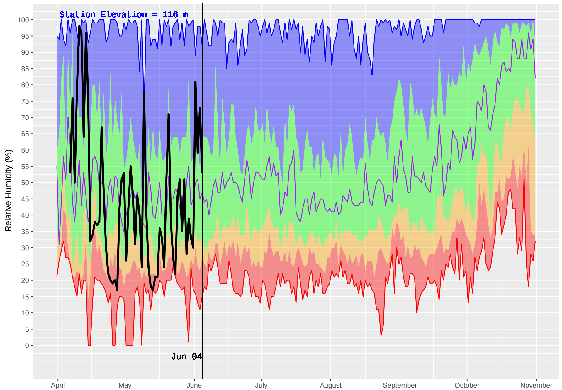
SCAR CREEK (82) : Historical (1982–2016) and Current (2018) Noon Relative Humidity
