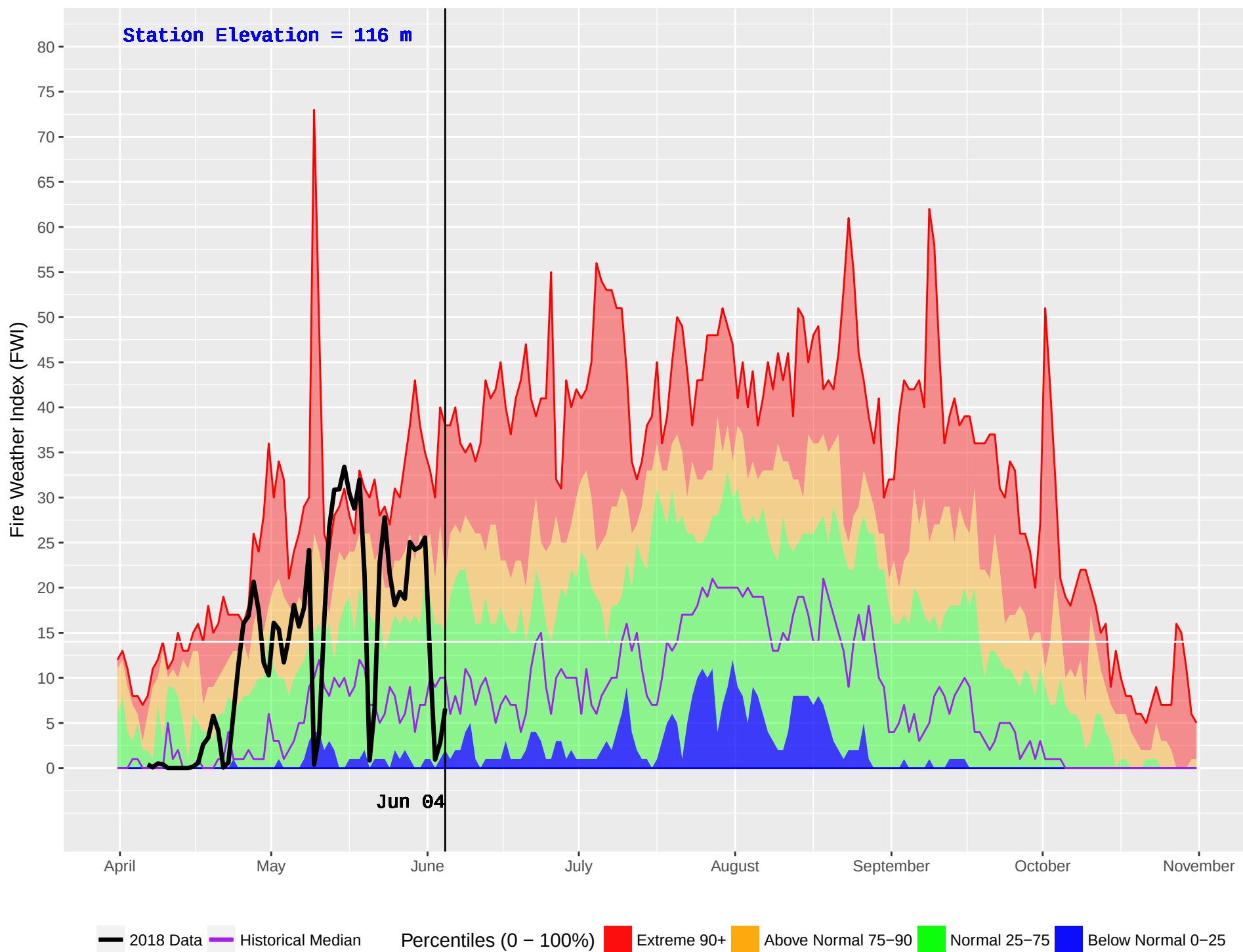
SCAR CREEK (82) : Historical (1982–2016) and Current (2018) Noon Fire Weather Index (FWI)
